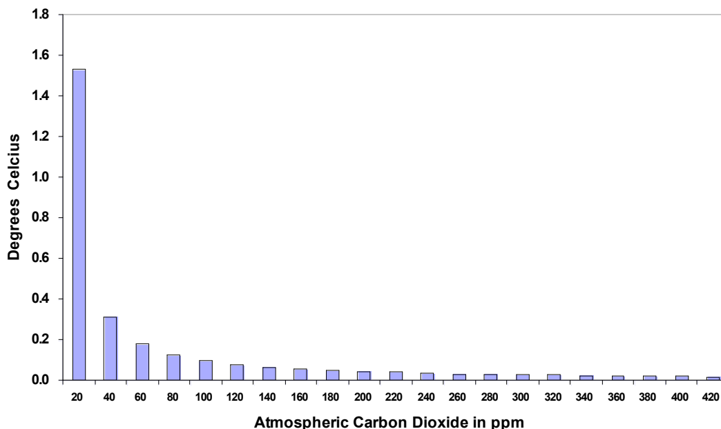
Figure 22: The Warming Effect of Carbon Dioxide
