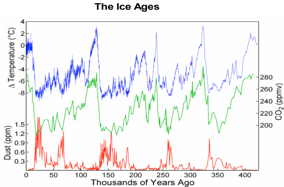
Figure 7: The Last Four Ice Ages
