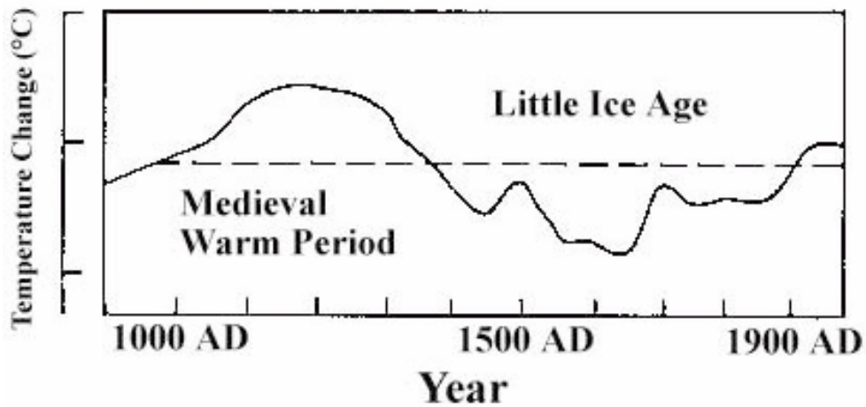
Figure 5: 1990 IPCC Chart of the Medieval Warm Period – Little Ice Age
