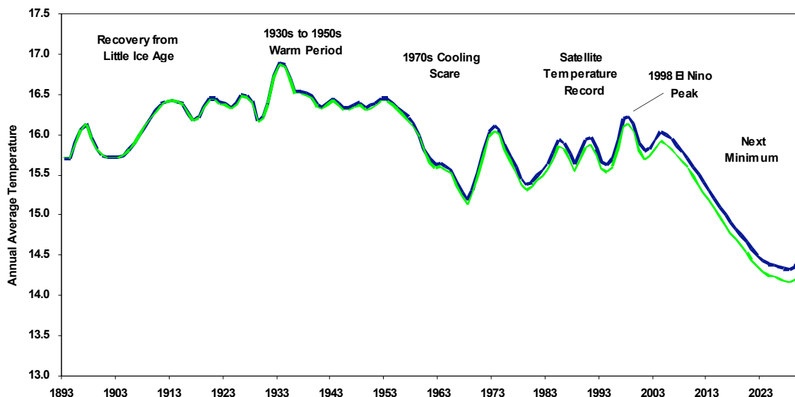
Figure 26: Calculated Anthropogenic Contribution to Atmospheric Temperature 1893 - 2030
