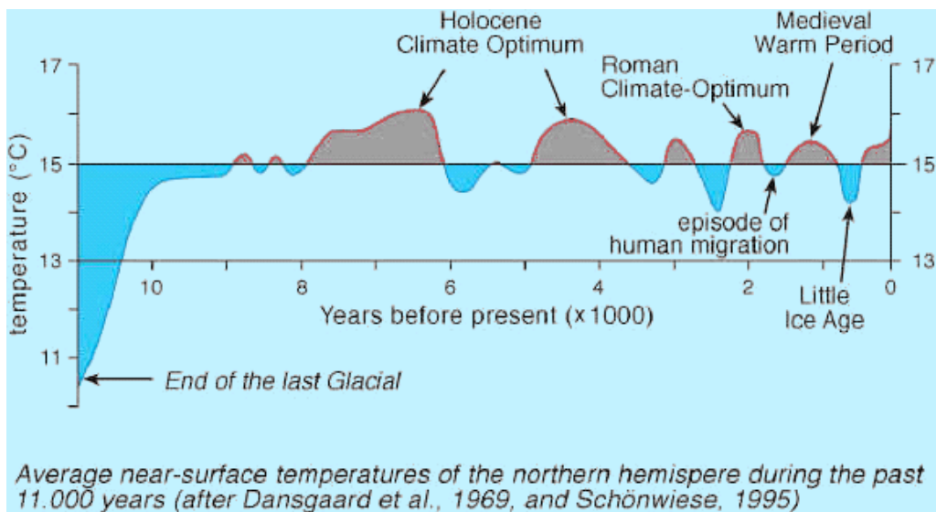
Figure 6: The Holocene Optimum
