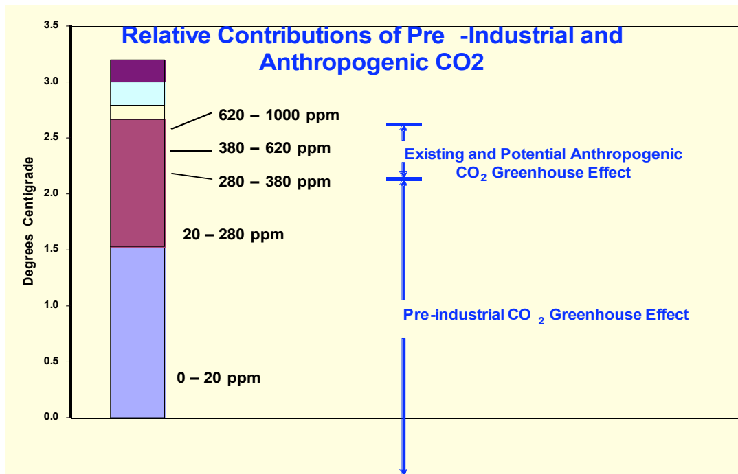
Figure 23: Relative Contributions of Pre-Industrial and Anthropogenic CO2
