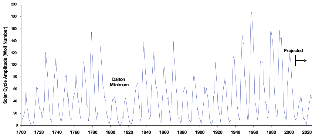
Figure 10: Sunspot Cycles 1700 - 2030
