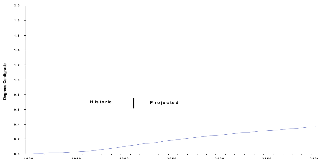
Figure 24: Atmospheric Temperature Increase due to Carbon Dioxide 1900 - 2200
