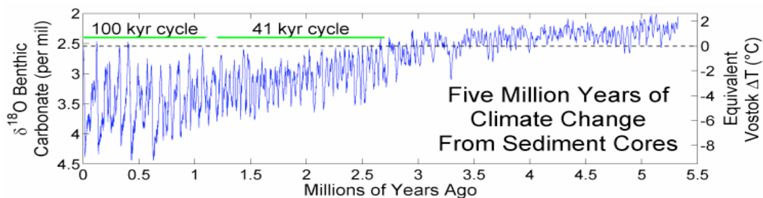
Figure 8: Ice Ages over the last 5.5 million years
