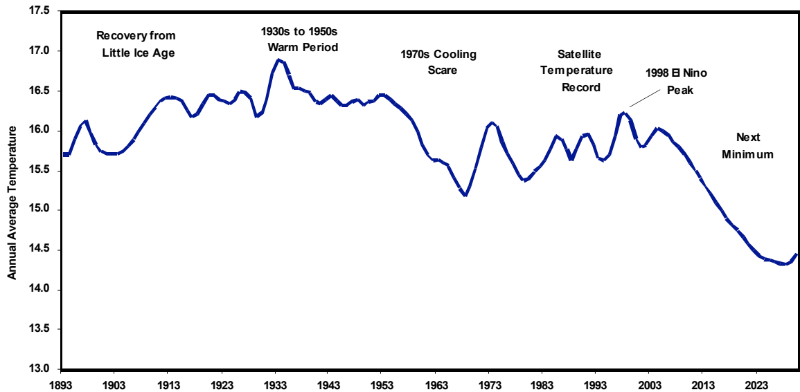
Figure 20: Projected Temperature Profile to 2030
