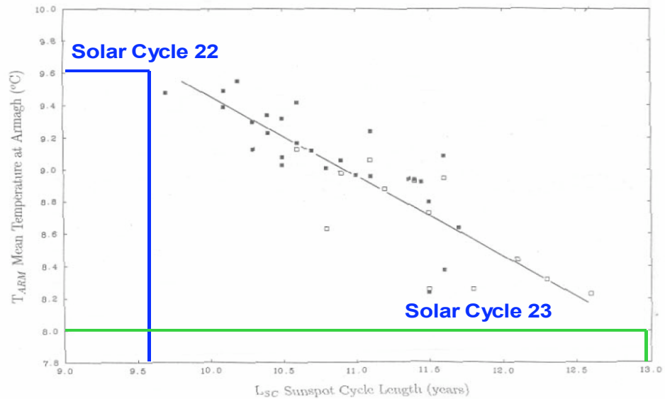
Figure 5. The mean temperature at Armagh for 11 year intervals, centred on years of sunspot maximum and minimum, plotted against the sunspot cycle length. Symbols: open squares - Series I, filled squares - Series II. The mean regression line is shown.
