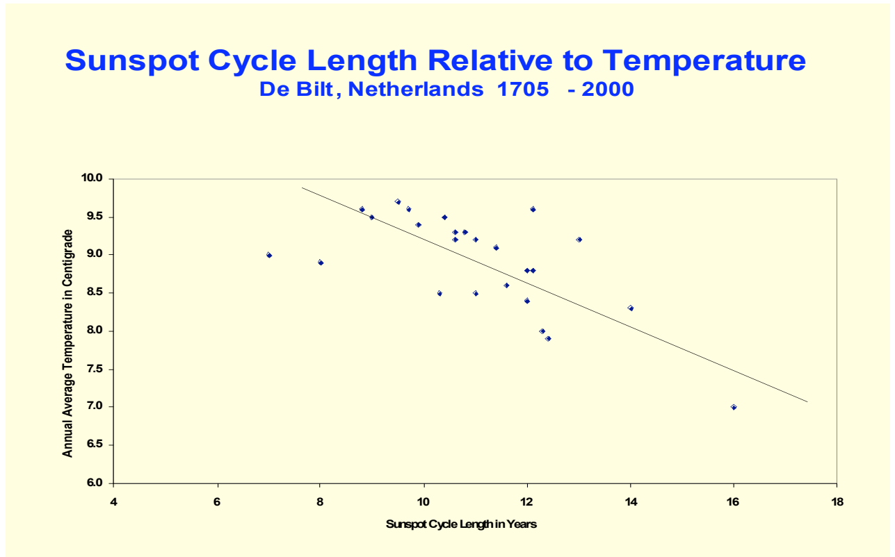
Figure 12: Sunspot Cycle Length Relative to Temperature – De Bilt
