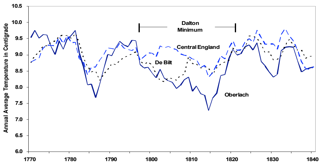
Figure 11: The Dalton Minimum in Europe
