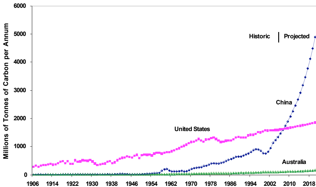
Figure 25: Historic and Projected Atmospheric Carbon Contributions by the United States, China and Australia
