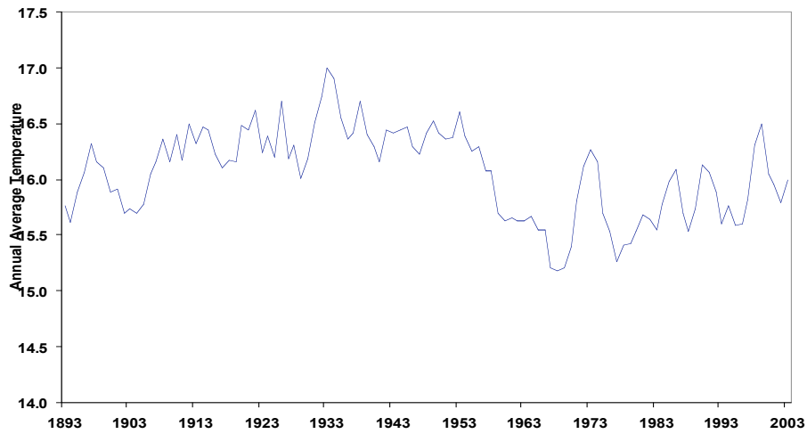
The smoothed average annual temperature of the Hawkinsville (32.3N, 83.5W), Glennville (31.3N, 89.1W), Calhoun Research Station (32.5N, 92.3W), Highlands (35.0N, 82.3W) and Talbotton (32.7N, 84.5W) stations is representative of the US temperature profile away from the urban heat island effect over the last 100 years (Data source: NASA GISS)
