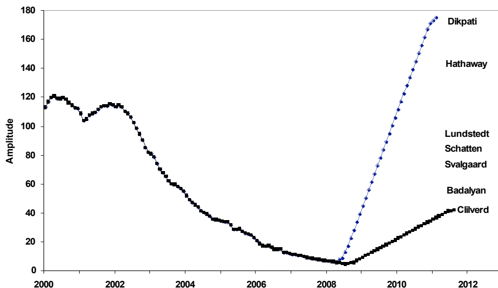
Figure 18: Predictions of Solar Cycle 24
